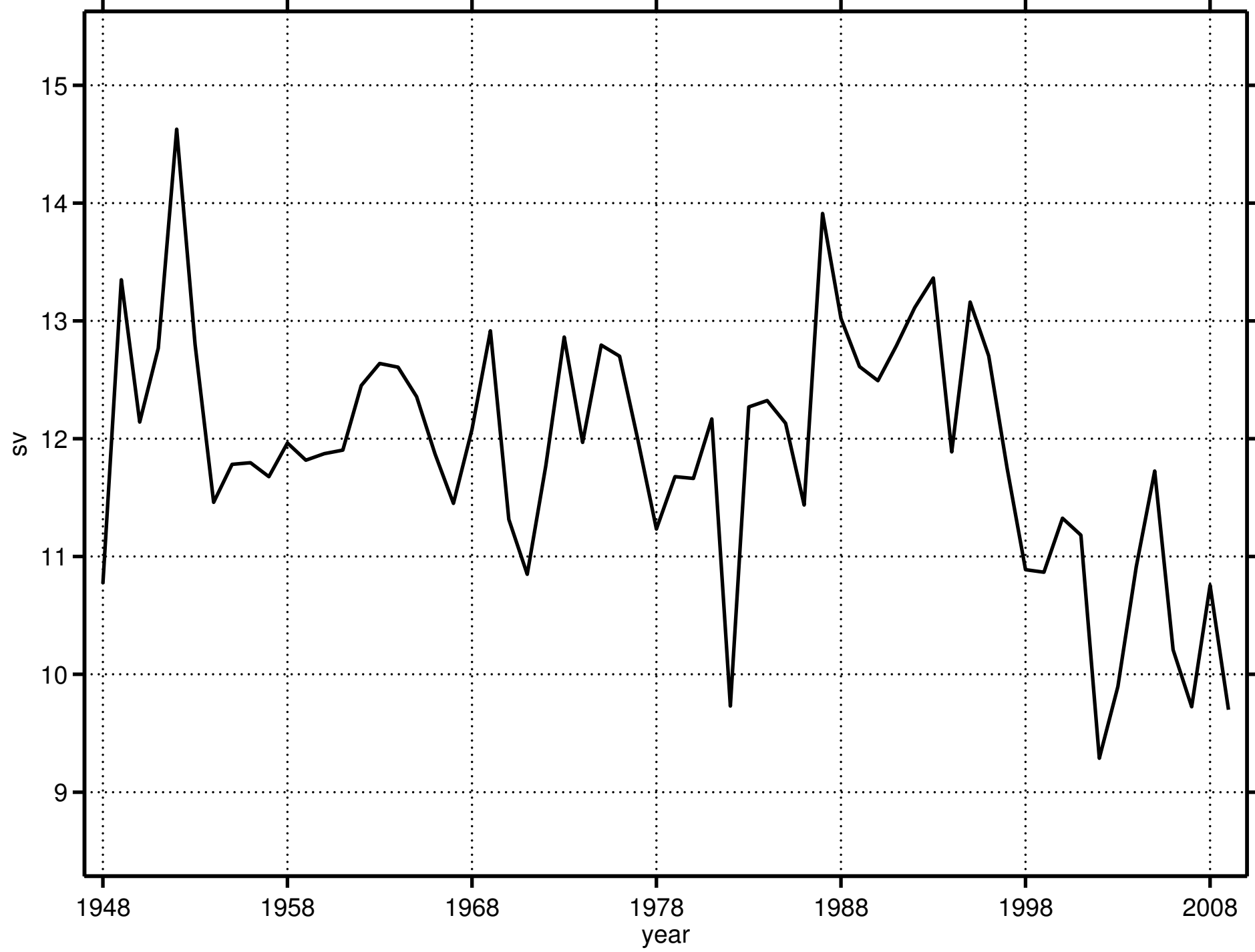
Maximum (20N–50N) Atlantic Meridional Overturning
