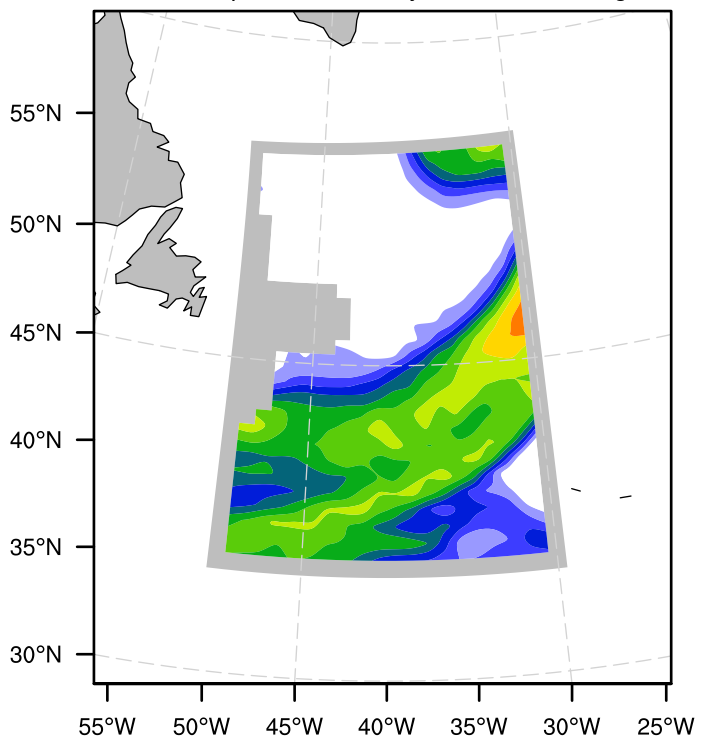
Gradient of potential density @500m 1e-6 \text{ kg/m}^3
