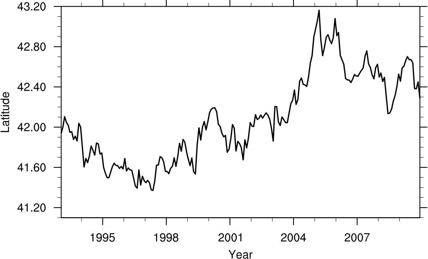
Subpolar Front index
