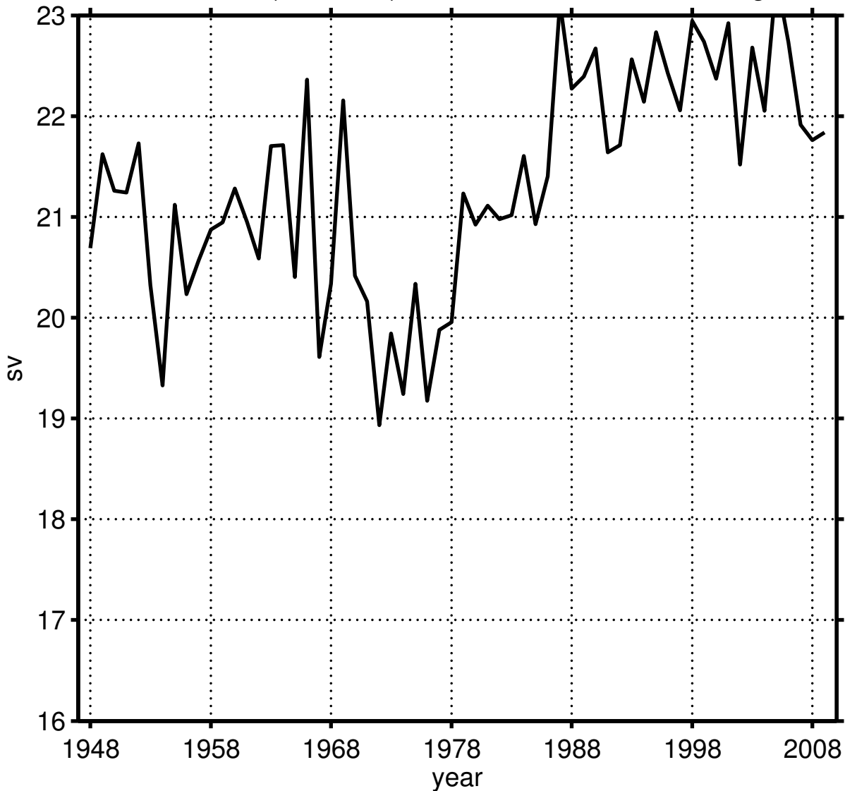
Maximum (20N–50N) Atlantic Meridional Overturning
